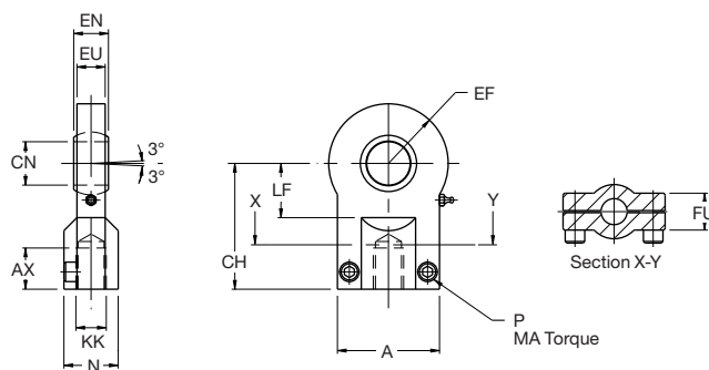
Spherical rod eye conforms to ISO 8133/DIN 24 555
